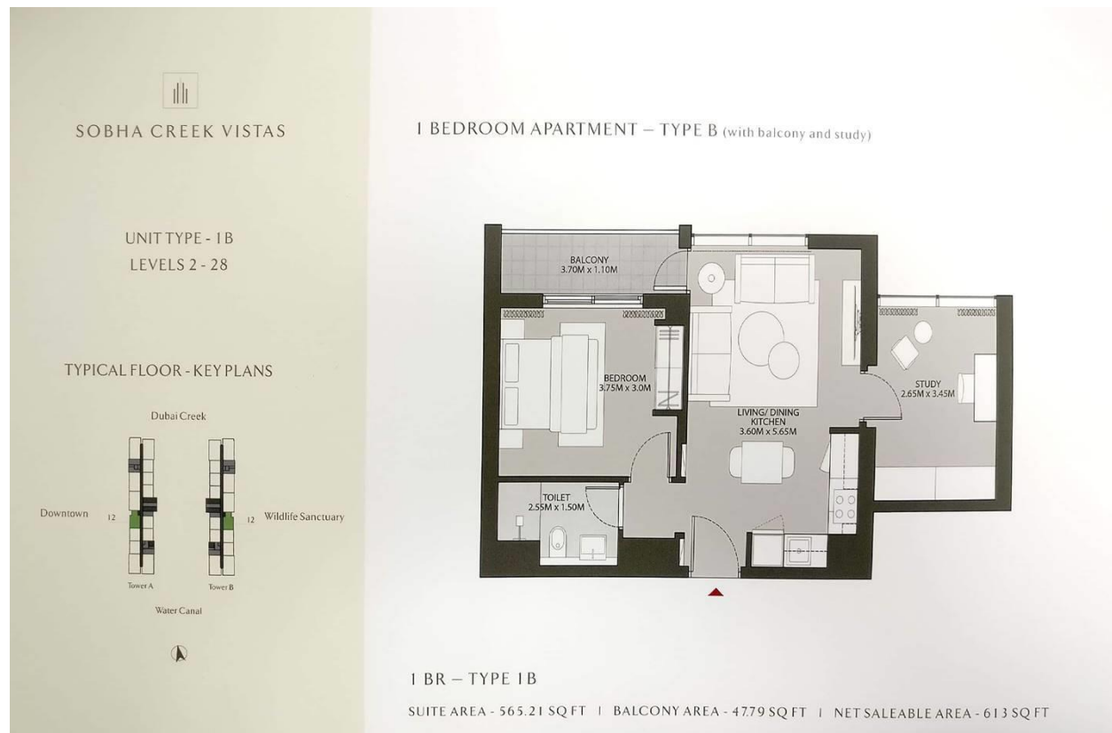
Figure 7 Layout: 1 Bedroom :
